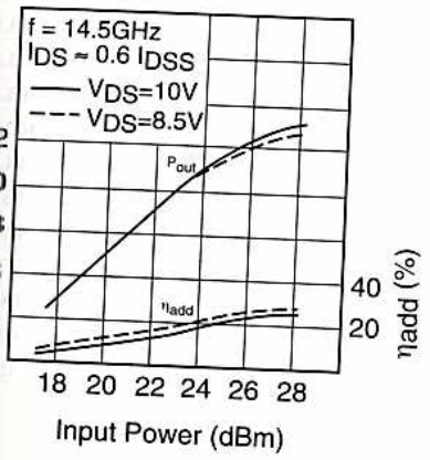
OUTPUT POWER vs. INPUT POWER
